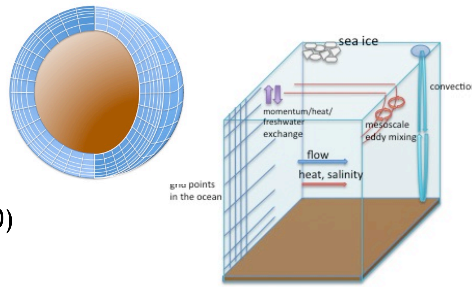
Figure 2: Schematic figure for (left) a model grid, and (right) processes included in the model.
