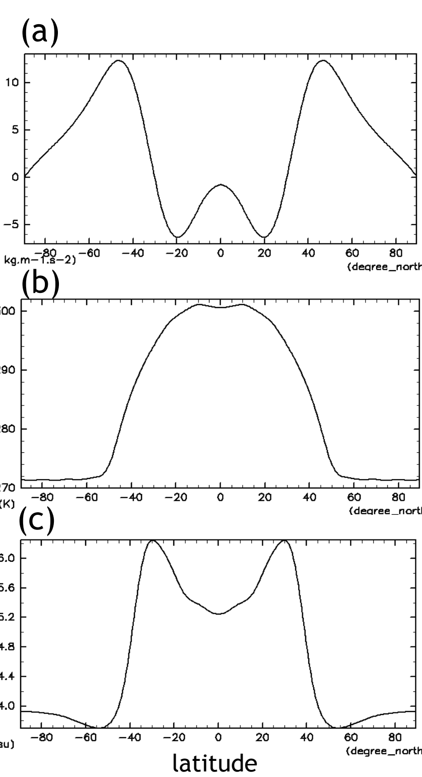
Figure 3: Meridional distribution of surface (a) stress (in N/m 2 ), (b) temperature (in K) and (c) salinity (in psu).
